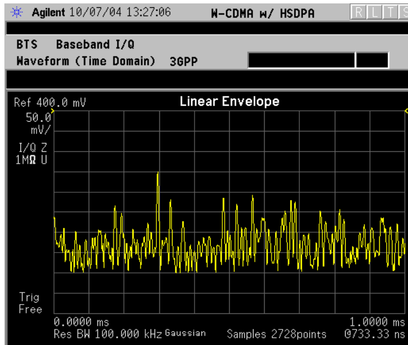
Figure 3-32 Waveform Measurement - Linear Envelope View
