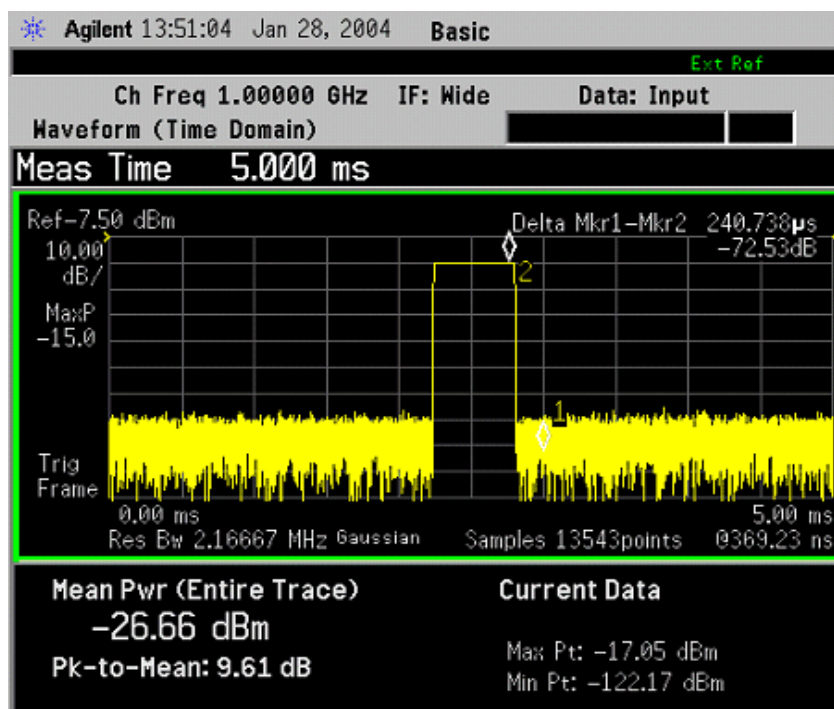
Figure 2-65 Waveform Measurement - RF Envelope View with Opt. 122–80 MHz Bandwidth Digitizer Hardware
