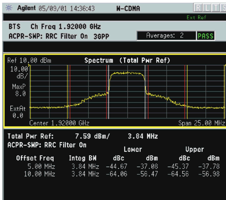
Figure 2-4 ACPR- SWP Measurement Result - Spectrum Graph View
