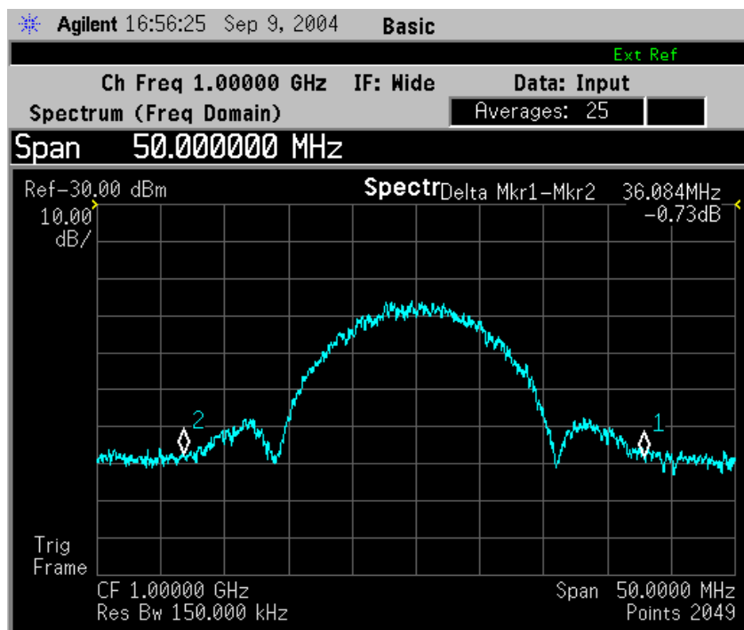
Figure 2-52 Spectrum Measurement - Spectrum Zoom View with Opt. 122–80 MHz Bandwidth Digitizer Hardware
