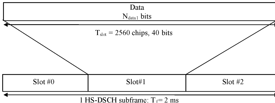
Figure 5-14 Subframe Structure of HS-SCCH
