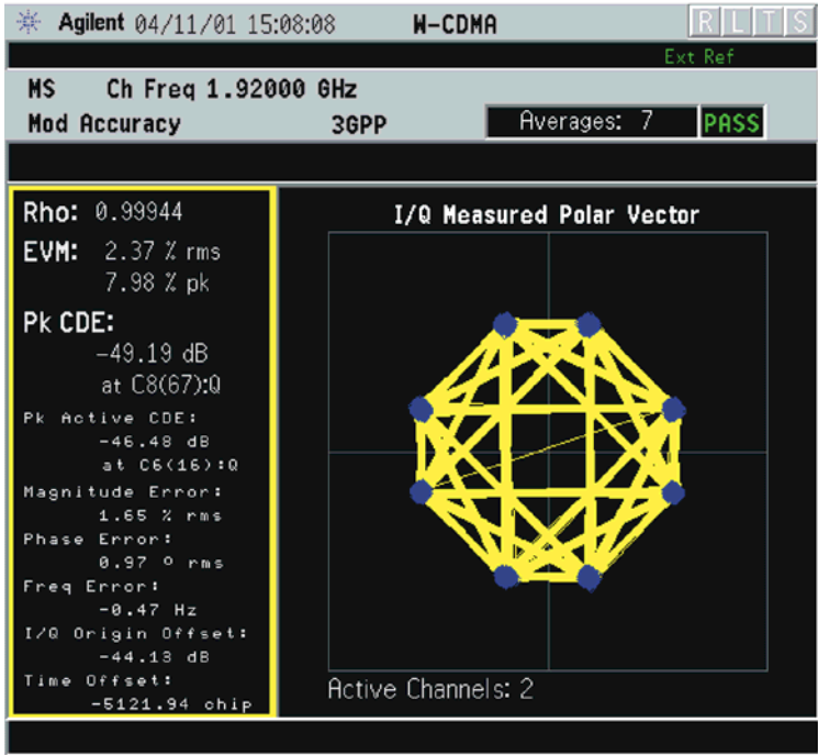
Figure 2-24 Modulation Accuracy Measurement Result - Polar Graph (Default) View
