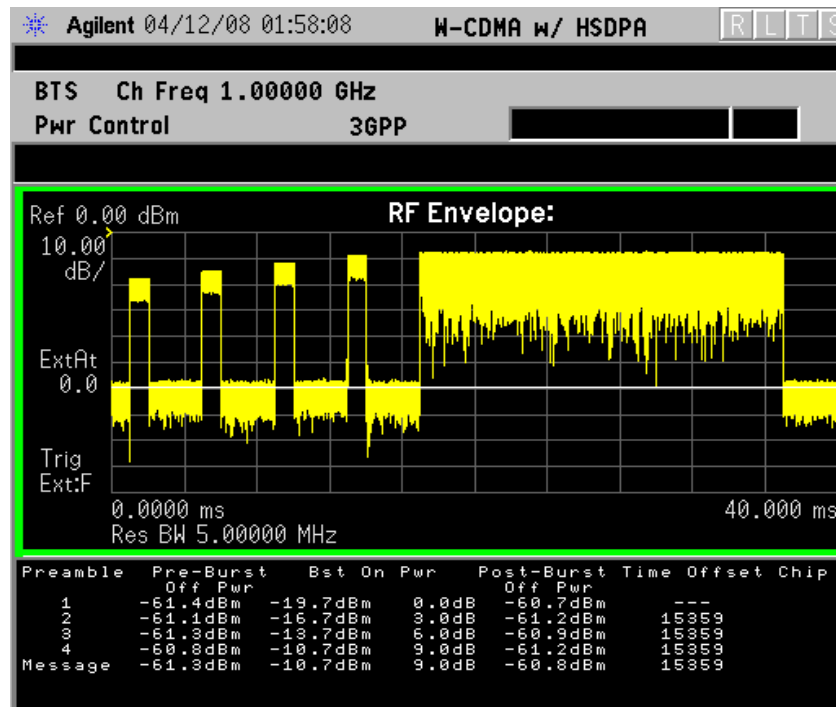
Figure 3-20 Power Control Measurement Result - PRACH Power Type
