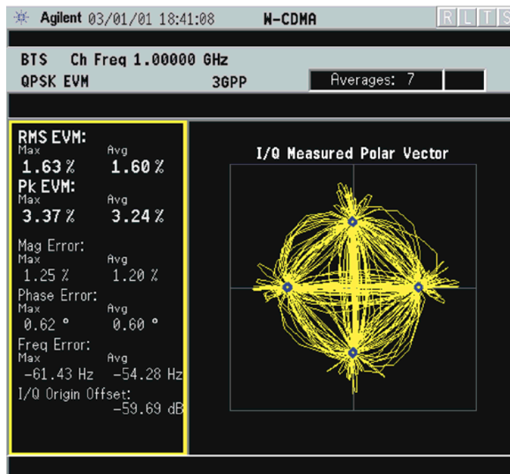
Figure 3-24 QPSK EVM Measurement - I/Q Measured Polar Graph
