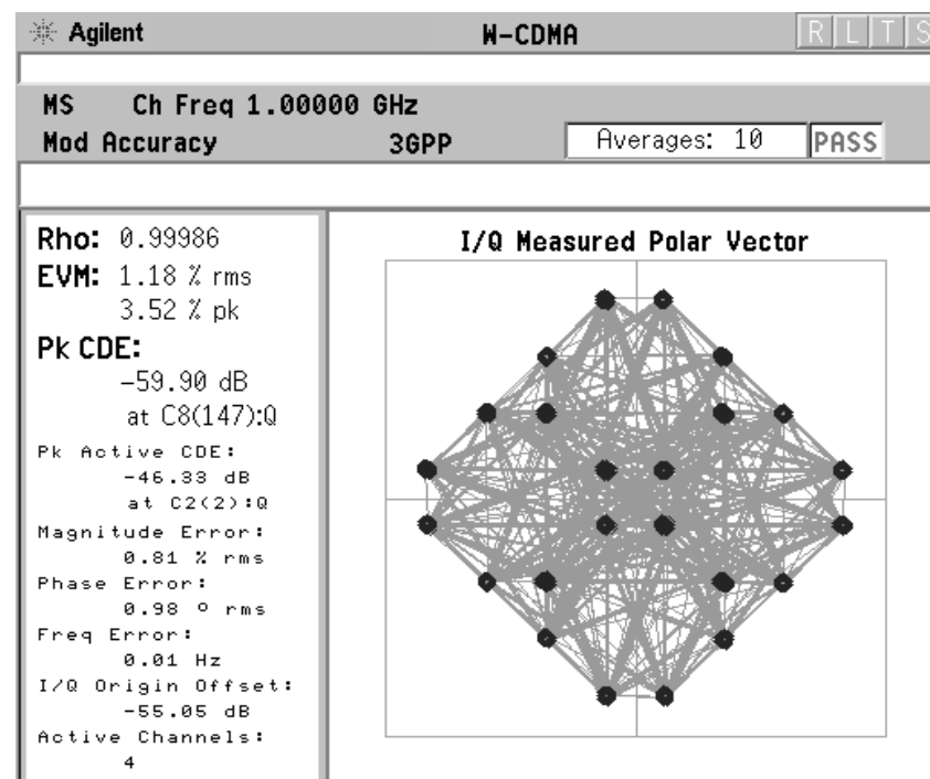
Figure 5-36 Composite EVM and Vector Diagram for a W-CDMA UL Signal with 12.2 kbps Reference Measurement Channel (three DPDCHs and a DPCCH)
