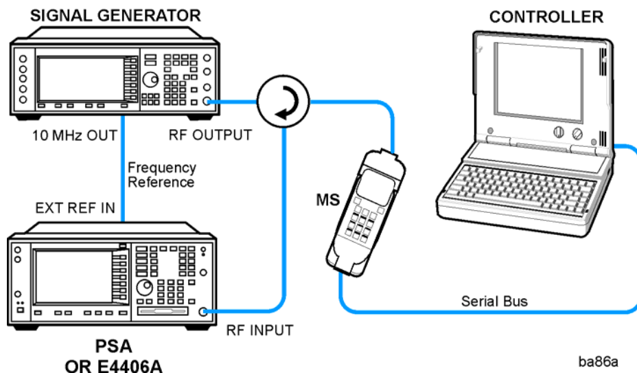
Occupied Bandwidth Measurement System
