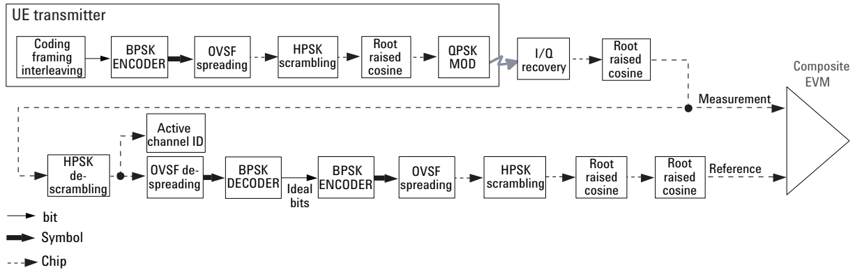
Figure 5-33 Process to Calculate Composite EVM for W-CDMA UL Signal
