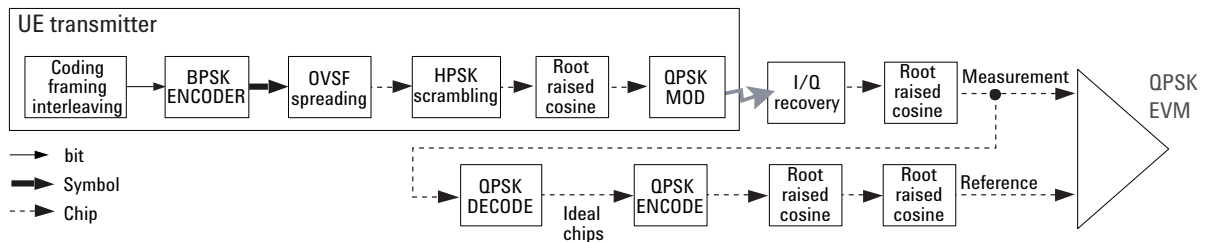
Figure 5-41 Process to Calculate QPSK EVM for a W-CDMA UL Signal
