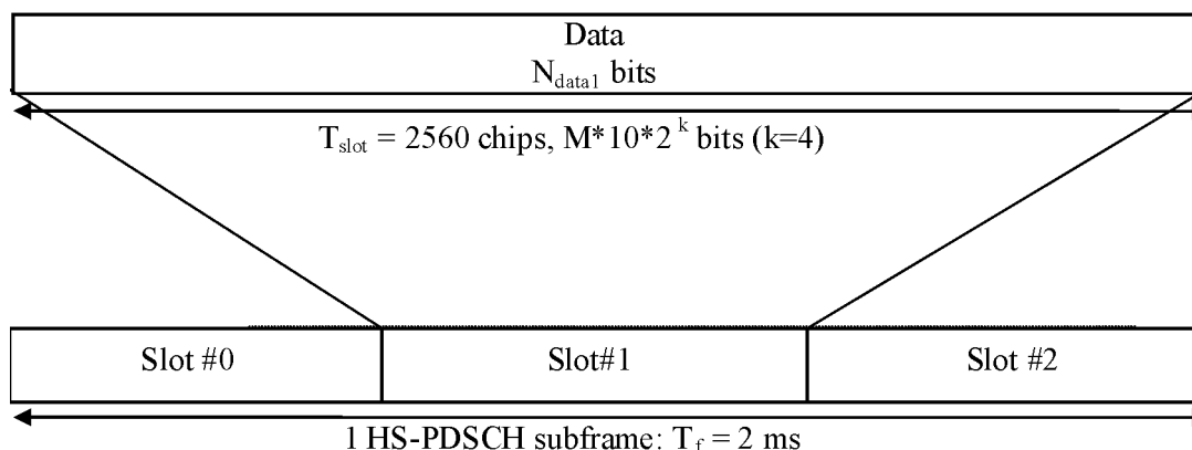
Figure 5-16 Subframe Structure for HS-PDSCH
