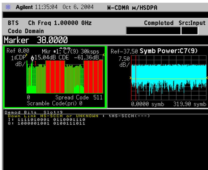
Figure 2-17 Code Domain Measurement Result - Demod Bits View - HSDPA DL Test Model 5
