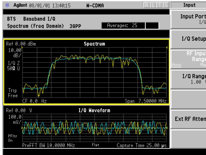
Figure 3-36 Input Menu with Option B7C Baseband I/Q Inputs Installed
