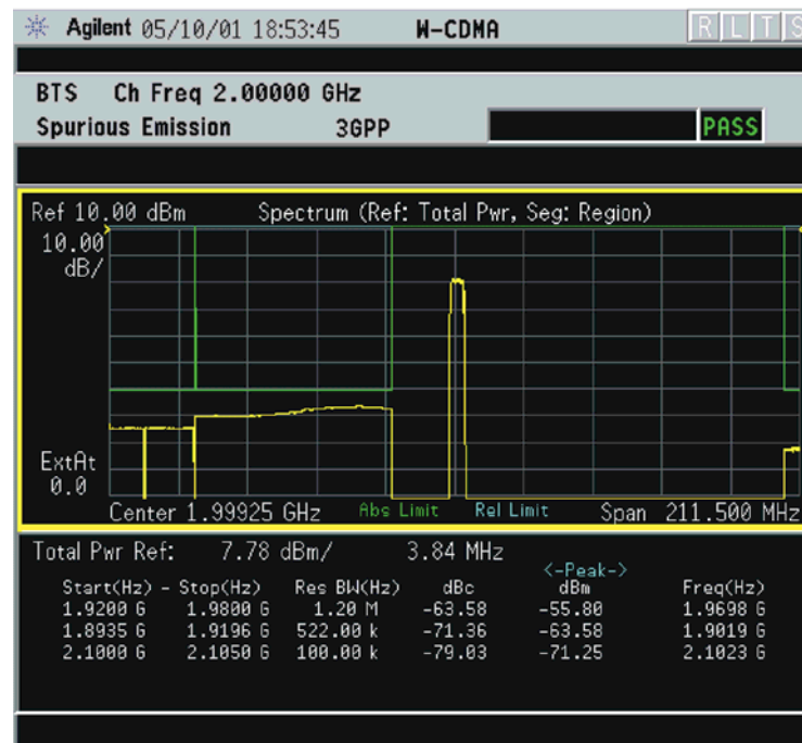
Figure 3-27 Spurious Emission Measurement - All Regions View
