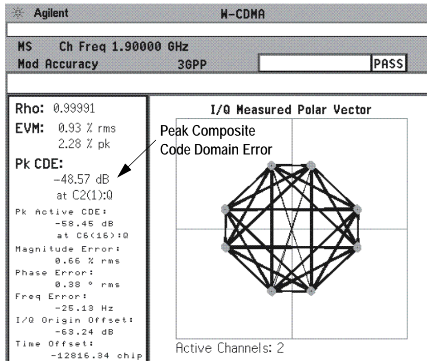
Figure 5-35 Composite EVM and Vector Diagram for a W-CDMA Signal with UL 12.2 kbps Reference Measurement Channel (one DPDCH and a DPCCH)
