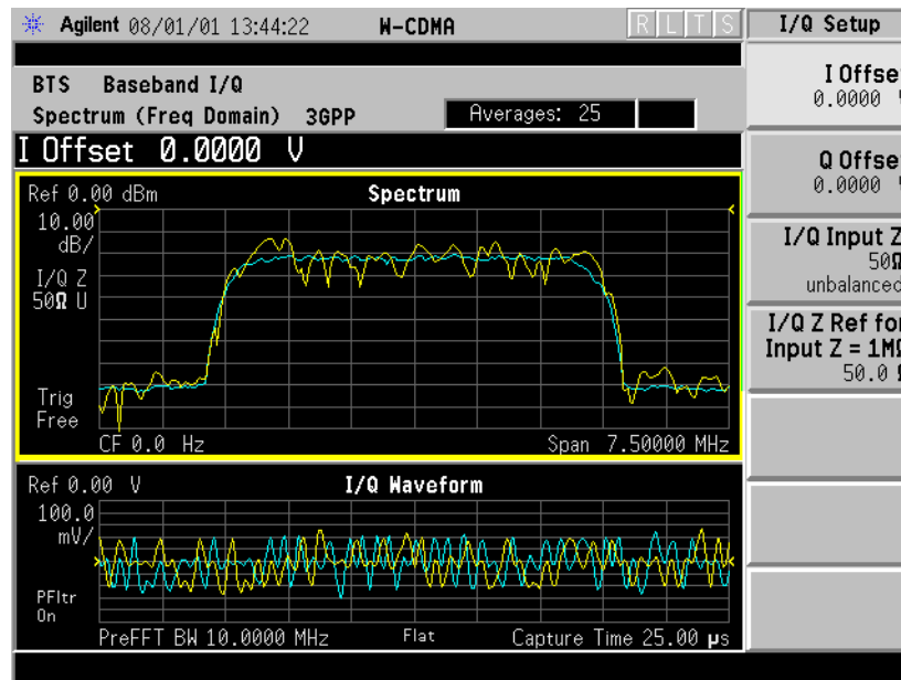
Figure 3-37 I/Q Setup Menu with Option B7C Baseband I/Q Inputs
