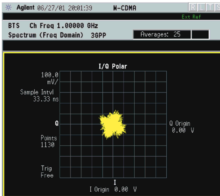
Figure 2-49 Spectrum Measurement - I/Q Polar View (for E4406A)
