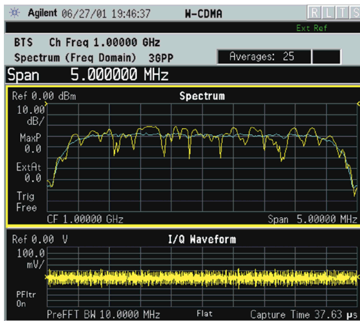
Figure 2-44 Spectrum Measurement - Spectrum and I/Q Waveform (Default View)
