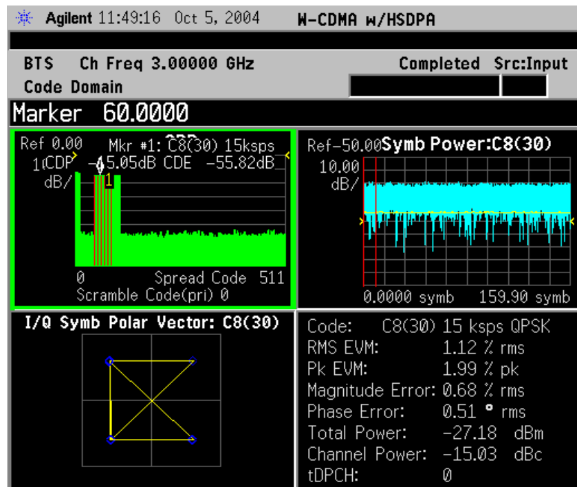
Figure 3-12 Code Domain Measurement - Code Domain Quad View
