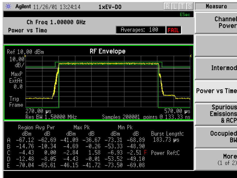
Figure 3-22 Power vs. Time Measurement - All Regions View
