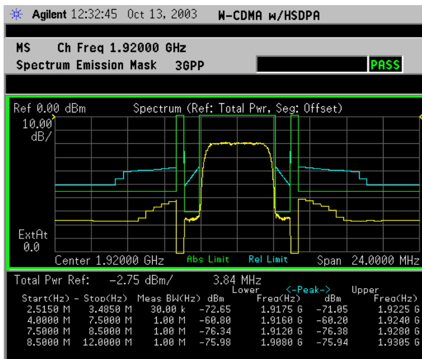
Figure 2-56 Spectrum Emission Mask Measurement Result - Offset Segment (Default) View
