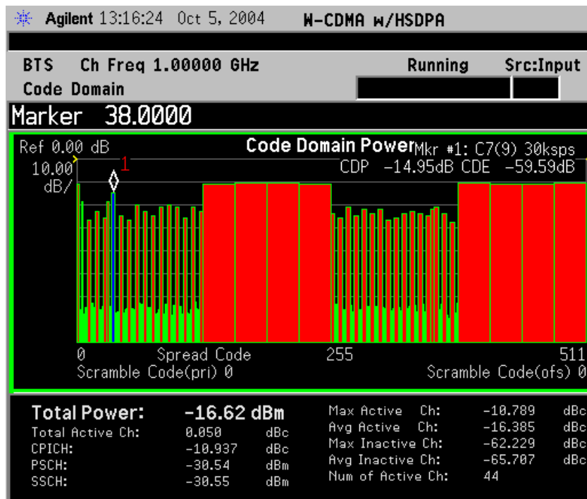
Figure 2-15 Code Domain Measurement Result - Power Graph and Metrics (Default) View - Downlink (BS) Test Model 5
