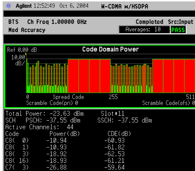
Figure 3-16 Modulation Accuracy Measurement - Code Domain Power
