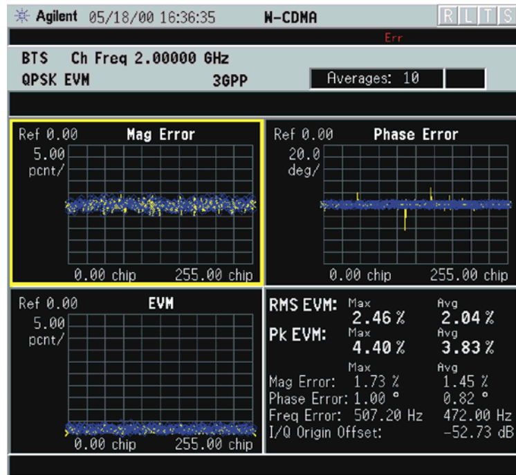
Figure 3-25 QPSK EVM Measurement - I/Q Error Quad View
