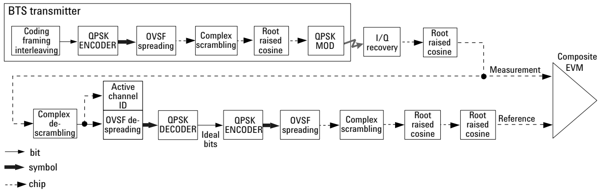
Figure 5-34 Process to Calculate Composite EVM for W-CDMA DL Signal
