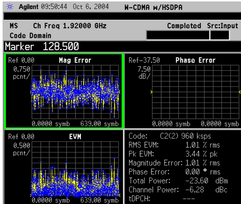
Figure 3-11 Code Domain Measurement - I/Q Error Quad View
