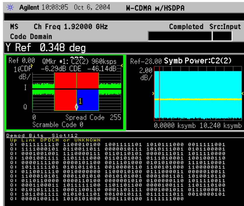
Figure 2-13 Code Domain Measurement Result - Demod Bits View
