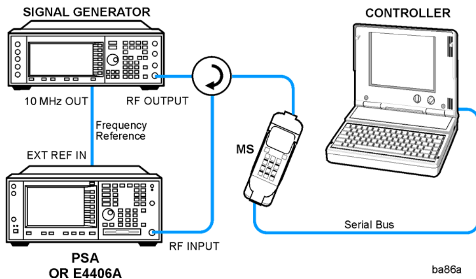
Figure 2-43 Spectrum Measurement System
