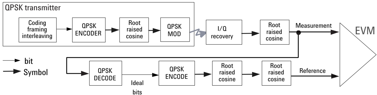
Figure 5-40 Process to Calculate EVM for a Generic QPSK Signal
