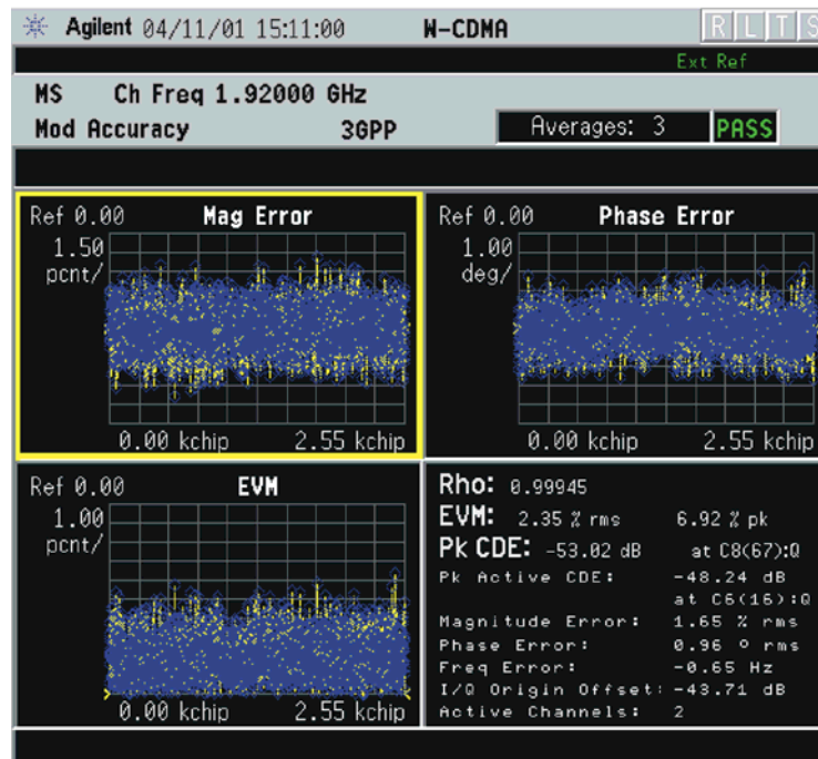
Figure 2-26 Modulation Accuracy Measurement Result - I/Q Error Quad View
