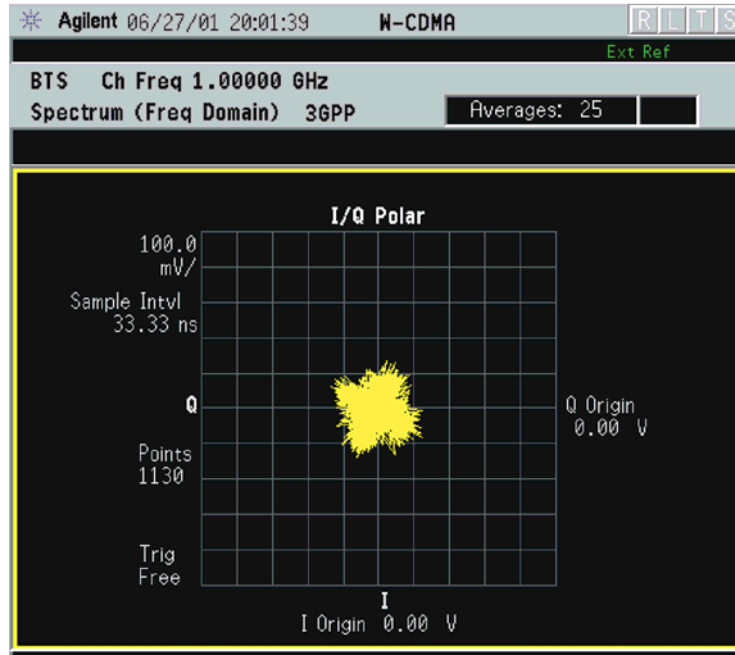
Figure 3-31 Spectrum Measurement - I/Q Polar View (for E4406A)
