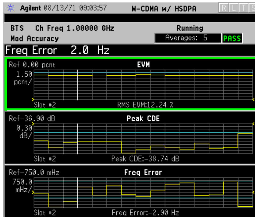
Figure 3-19 Mod Accuracy Measurement - Slot CDE/EVM View
