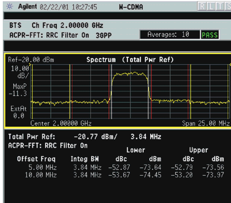
Figure 3-5 ACPR Measurement - FFT Spectrum (Total Pwr Ref) View
