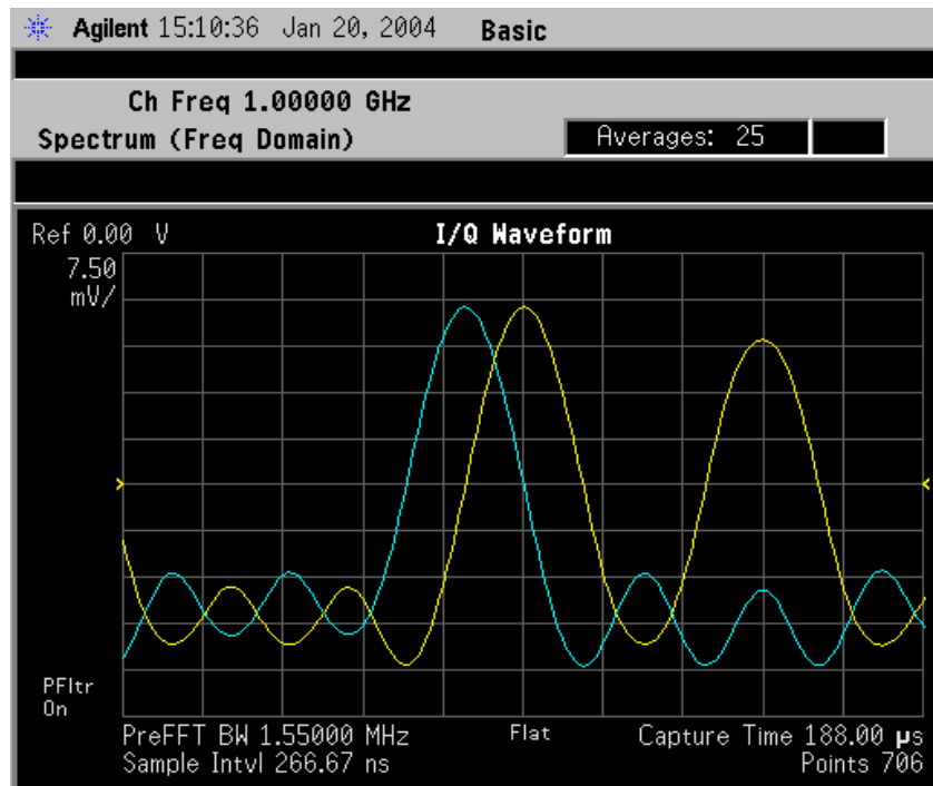
Figure 3-28 Spectrum Measurement - I/Q Waveform (Time Domain) Result (E4406A View)
