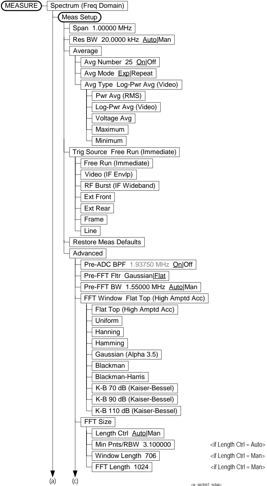
Figure 6-29 Spectrum (Freq Domain) Measurement Key Flow (1 of 4)
