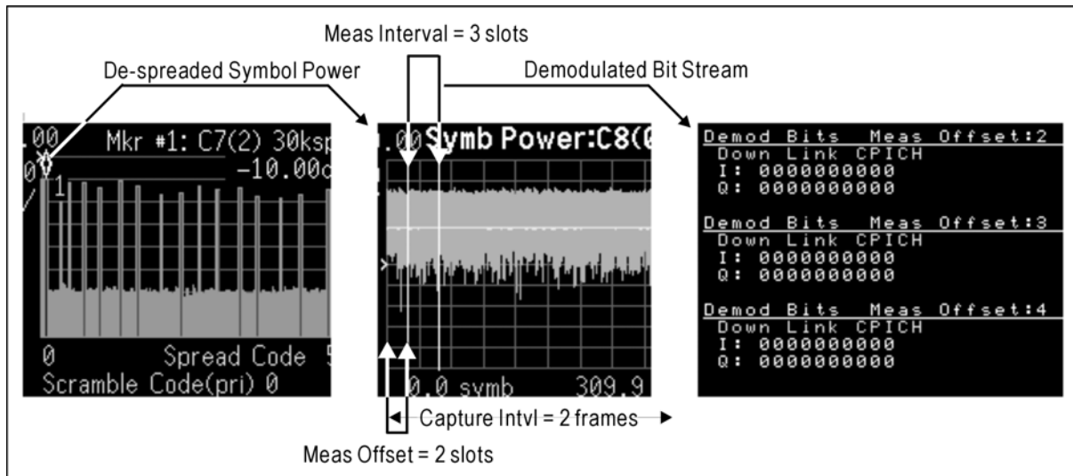
Figure 3-7 Capture Interval and Measurement Offset Parameters
