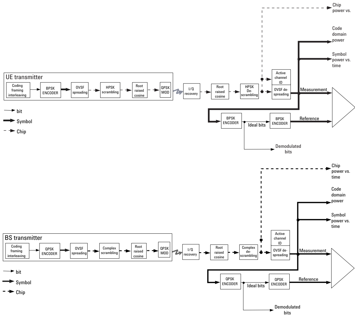
Figure 5-29 Process to Calculate Code Domain Power, Symbol EVM, Symbol Power vs. Time, Chip Power vs. Time, and Demodulated Bits US (UL) above, BS (DL) below
