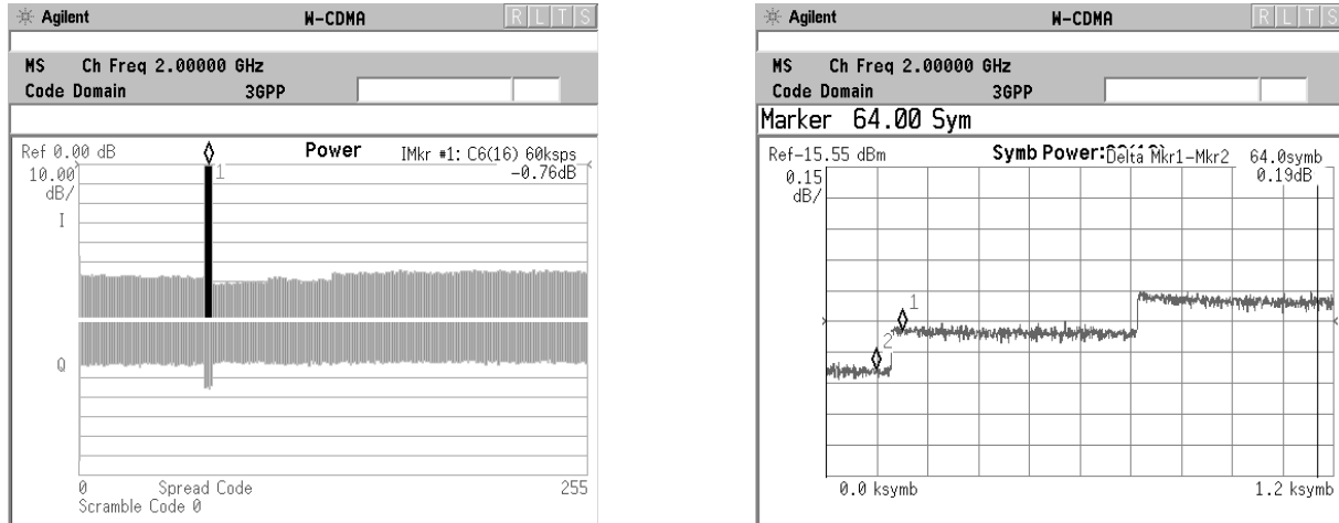
Figure 5-30 W-CDMA UL w/DPCCCH, one DPDCH at 60 kbps (Cch,64,16) CDP View (left) and Symbol EVM measurement View (right)
