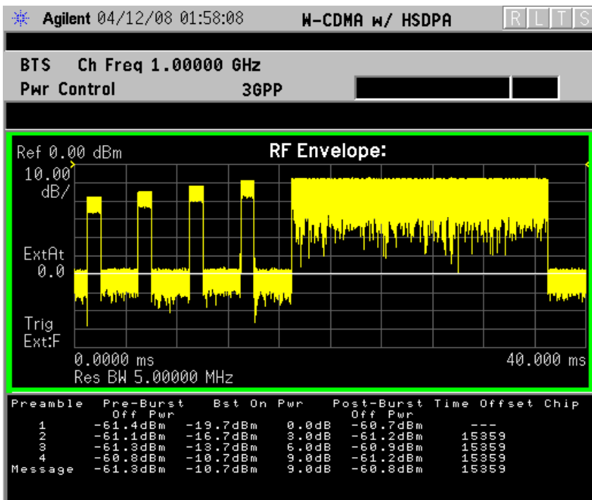
Figure 2-34 Power Control Measurement Result - PRACH Measurement
