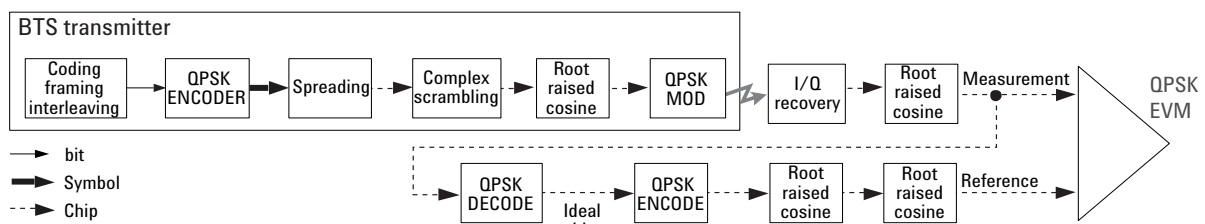
Figure 5-42 Process to Calculate QPSK EVM for a W-CDMA DL Signal
