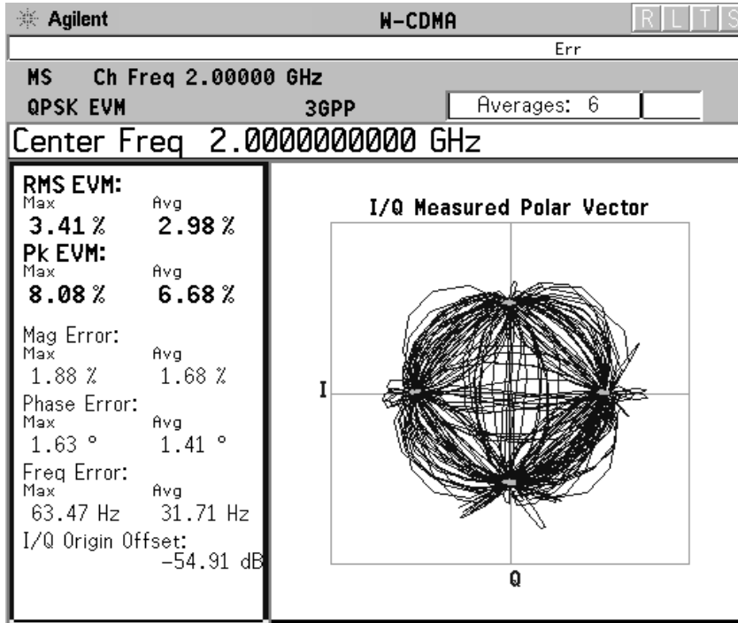
Figure 5-43 QPSK EVM Measurement of W-CDMA UL (without Impairment)
