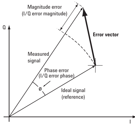
Figure 5-39 Error Vector and Related Parameters
