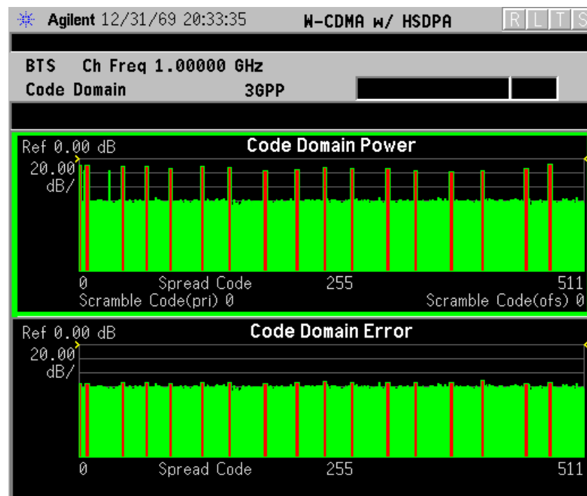
Figure 3-9 Code Domain Measurement - CDP Graph & CDE Graph (BTS)
