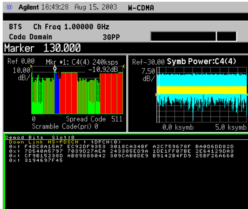
Code Domain Measurement Result - Demod Bits View (Hex)
