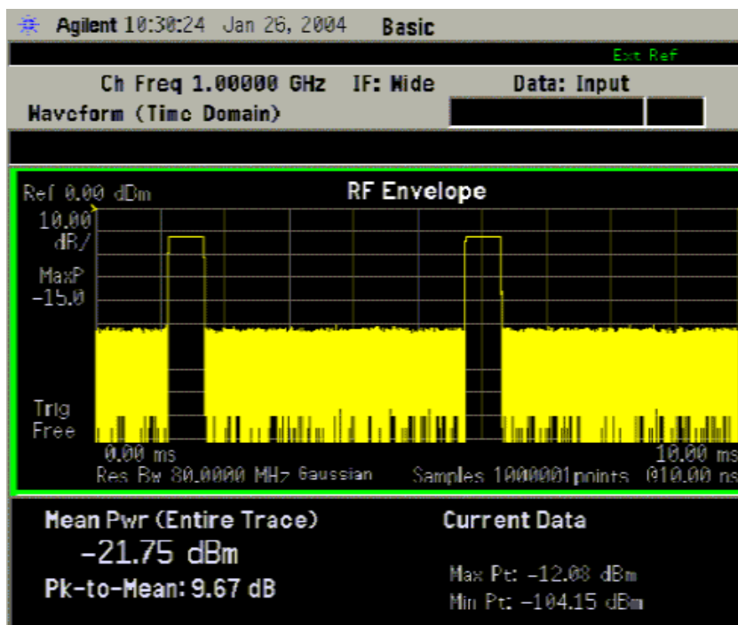
Figure 2-64 Waveform Measurement - RF Envelope View with Opt. 122– 80 MHz Bandwidth Digitizer Hardware
