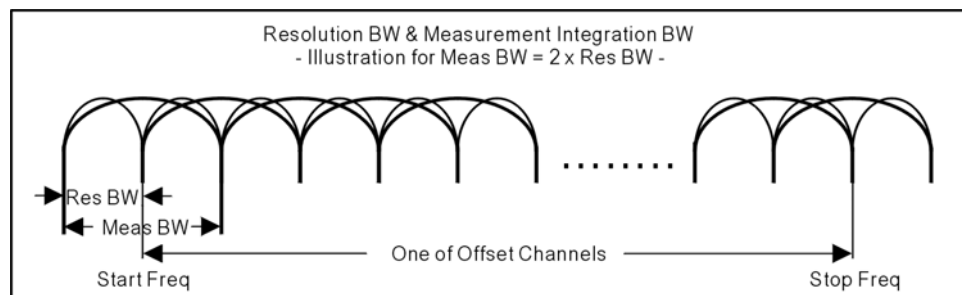
Figure 3-26 Resolution BW and Measurement Integration BW
