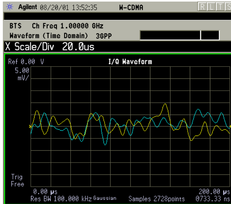
Figure 3-33 Waveform Measurement - I/Q Waveform View
