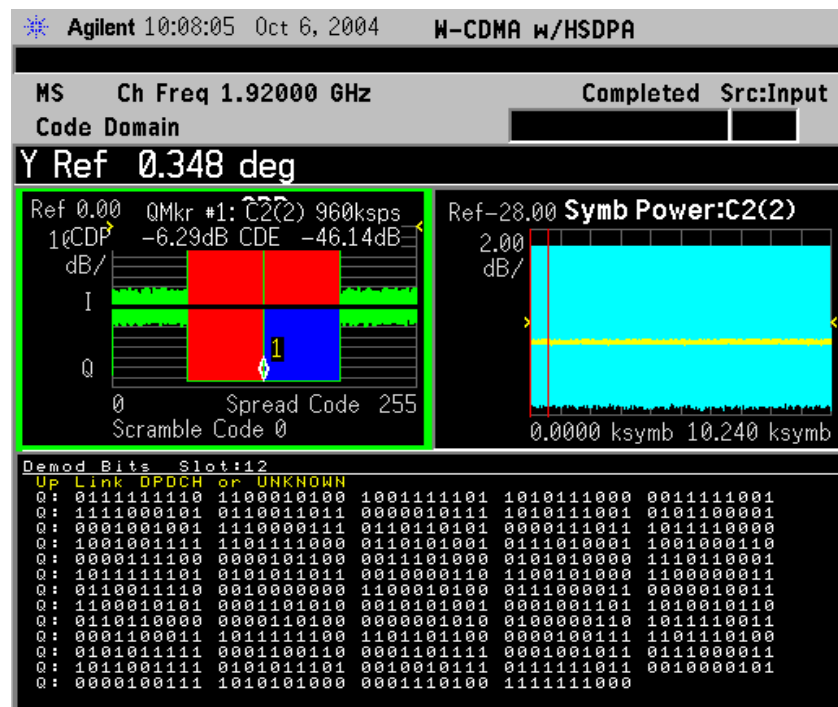
Figure 3-13 Code Domain Measurement - Demod Bits View (Single Slot)
