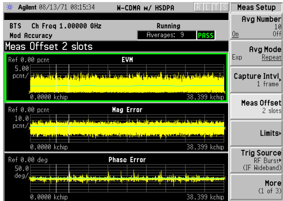
Figure 3-15 Modulation Accuracy Measurement - I/Q Error (Tri-View)
