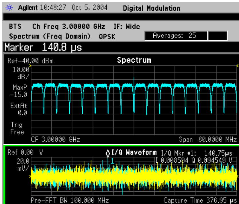
Figure 2-54 Spectrum Measurement - Spectrum Zoom View with Opt. 122–80 MHz Bandwidth Digitizer Hardware
