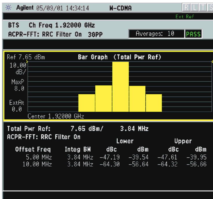
Figure 2-2 ACPR-FFT Measurement Result - Bar Graph (Default) View
