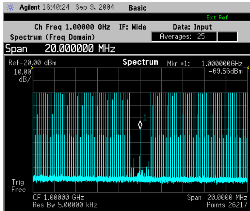
Figure 2-53 Spectrum Measurement - Spectrum View with Opt. 122– 80 MHz Bandwidth Digitizer Hardware
