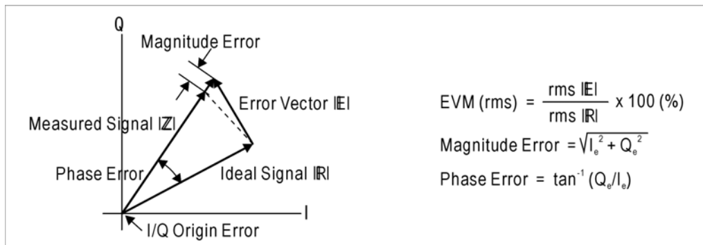
Figure 5-37 Error Vector Magnitude and Related Parameters
