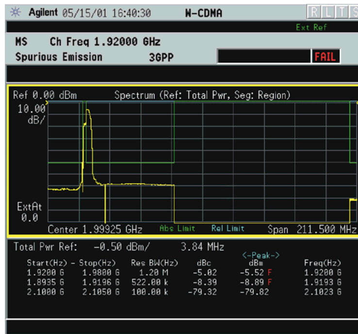
Figure 2-57 Spectrum Emission Mask Measurement Result - Region Segment
