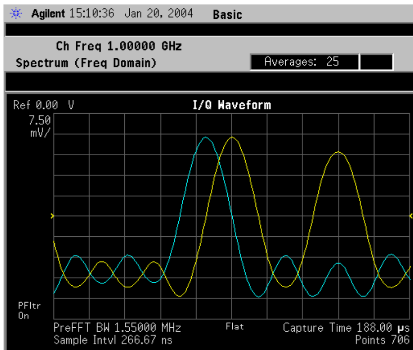
Figure 2-45 Spectrum Measurement - I/Q Waveform (Time Domain) Result (E4406A View)
