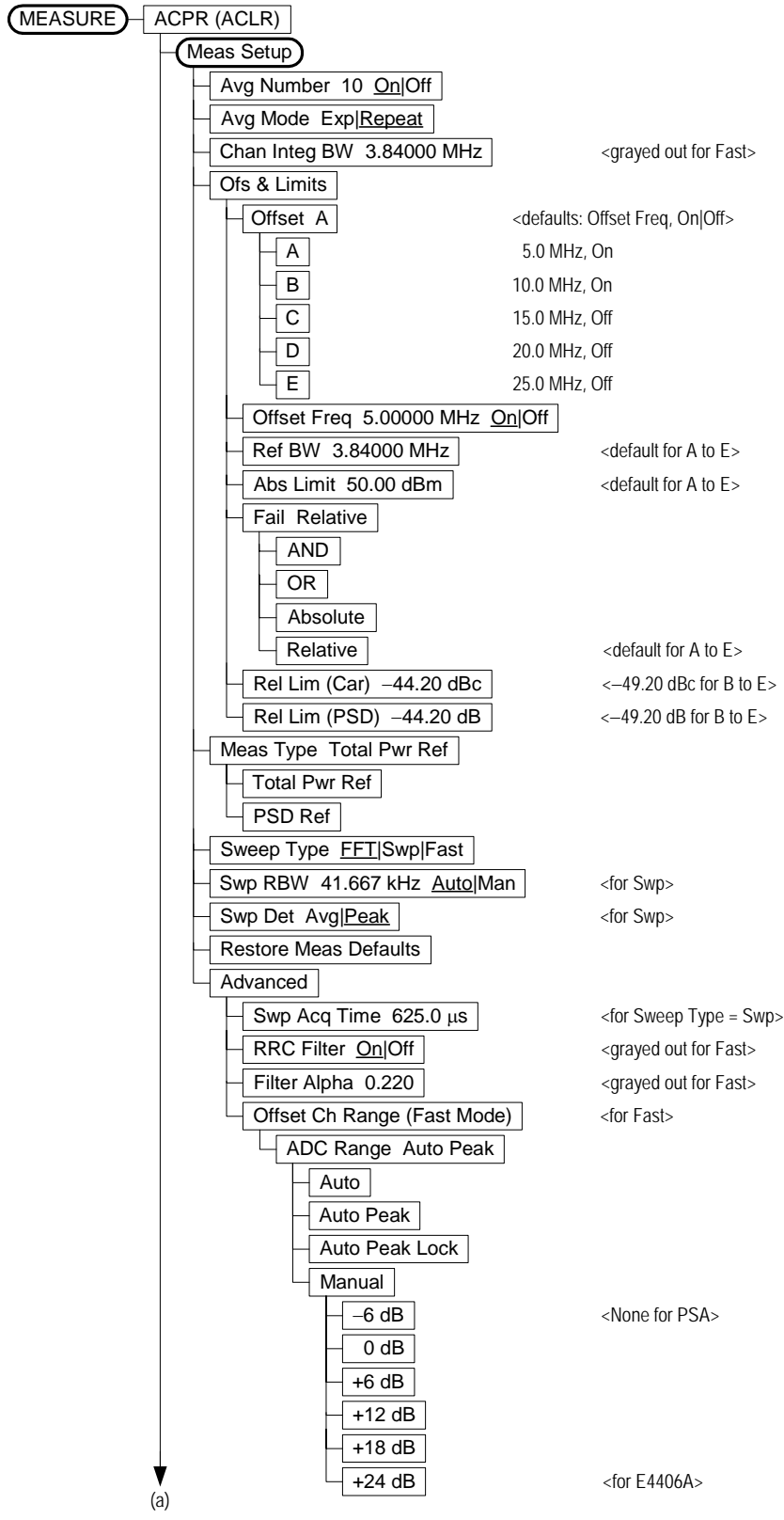
Figure 6-6 ACPR (ACLR) Measurement Key Flow (1 of 2)
