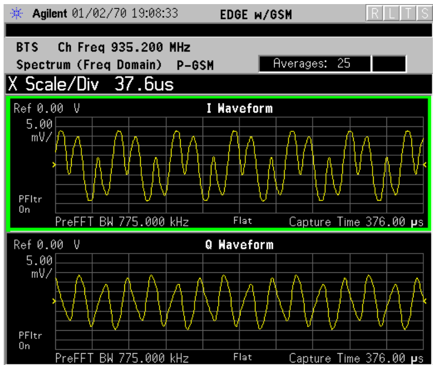
Figure 2-48 Spectrum Measurement - I and Q Waveform View (for E4406A)
