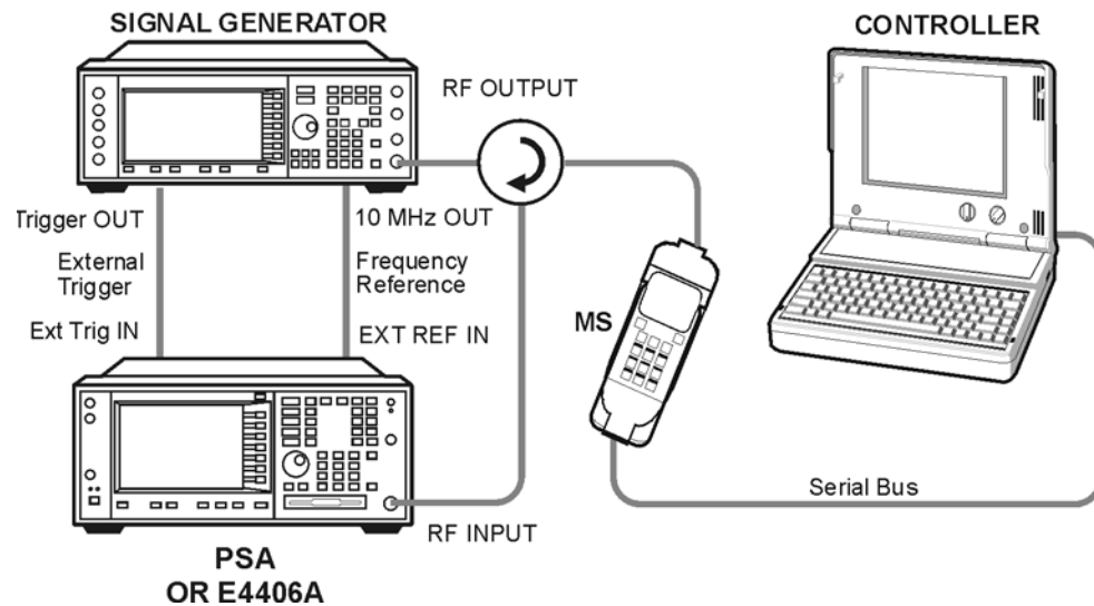
Figure 2-32 Power Control Measurement System
