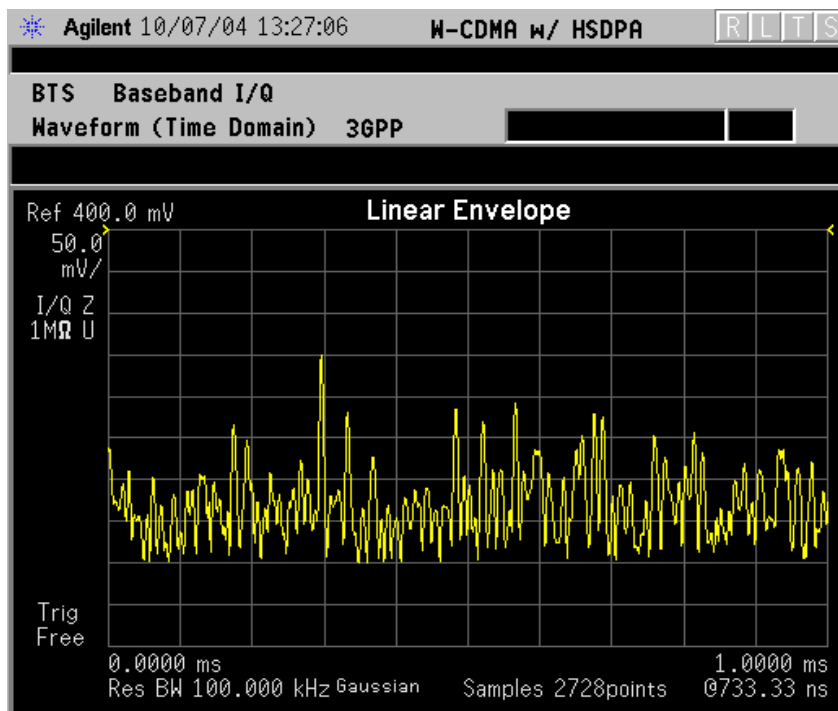
Figure 2-60 Waveform Measurement - Linear Envelope View
