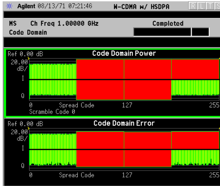
Figure 3-10 Code Domain Measurement - CDP Graph & CDE Graph (MS)
