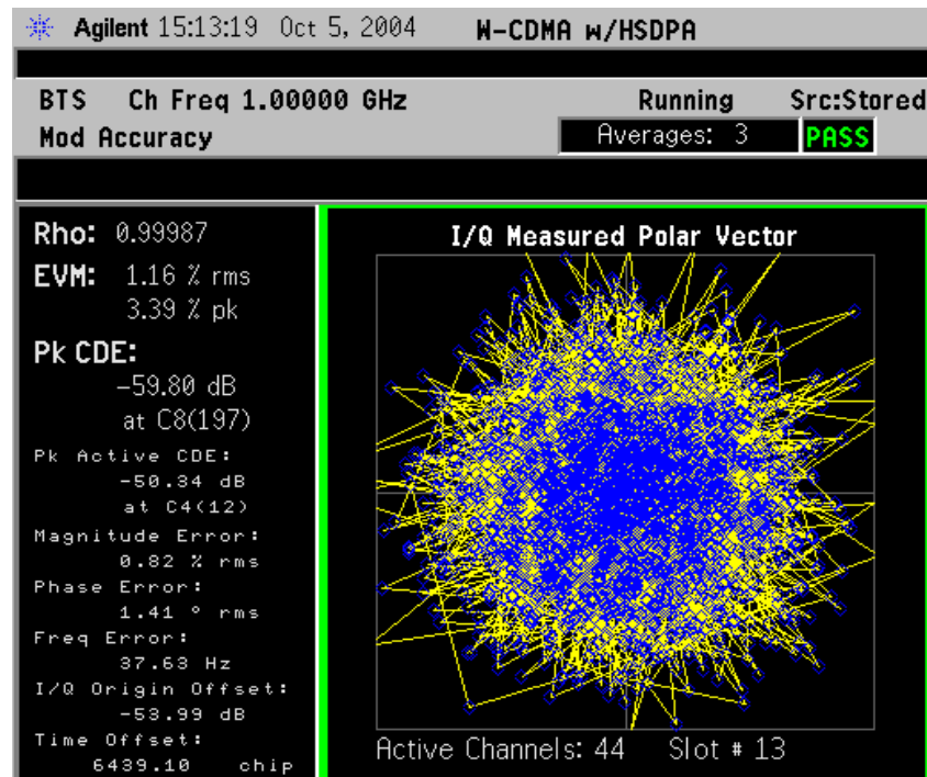
Figure 3-3 Mod Accuracy Measurement - (BTS) with Data Sharing Enabled “Src: Stored” Displayed at Top Right Corner
