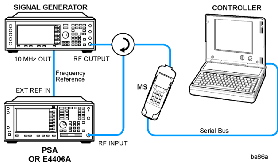
Figure 2-23 Modulation Accuracy Measurement System
