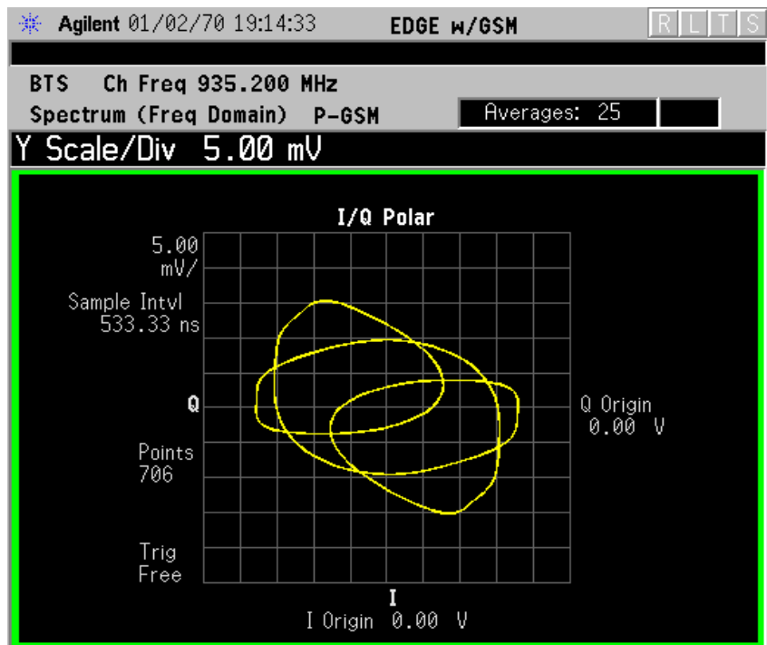
Figure 2-50 Spectrum Measurement - I/Q Polar View (for E4406A)
